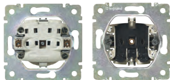
New screwless terminals for sockets.
